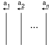
FIGURE 5. A p -adic identity framed braid
