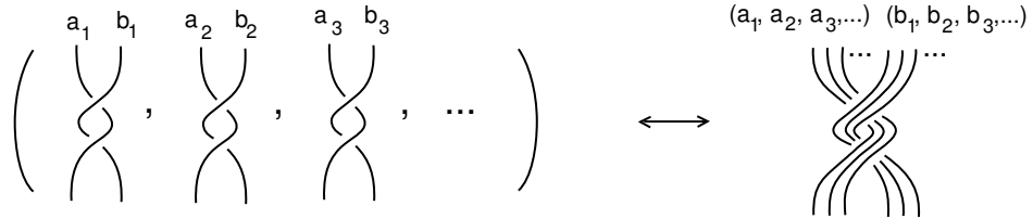
FIGURE 1. A p -adic framed braid as an infinite framed cabling
