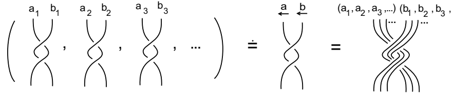
FIGURE 4. A p -adic framed braid
