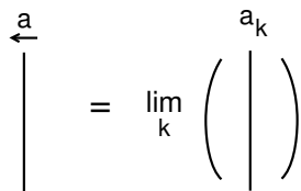
FIGURE 8. The approximation of an one-strand p -adic framed braid
