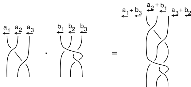
FIGURE 7. Multiplication of p -adic framed braids in \mathbb{Z}_p^n \rtimes B_n
