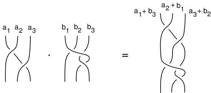
FIGURE 3. Multiplication of framed braids
