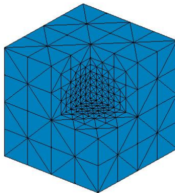
FIG. 5.4. Adaptive meshing for test problem 3
