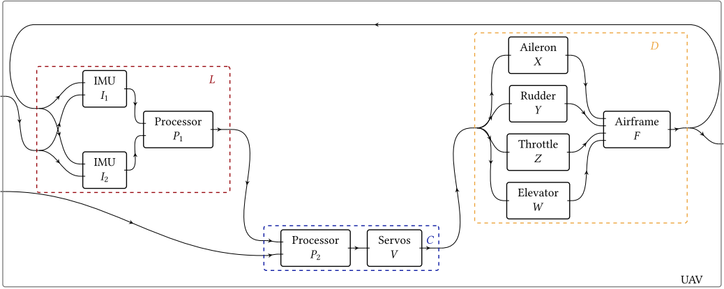
Fig. 4. Any decomposition, including the previous one (Figure 3) resides within the slice category \mathbf{W}/\text{UAV} . In this case, the slice category contains all possible design decisions that adhere to the behavioral model; we pick one such design choice.
