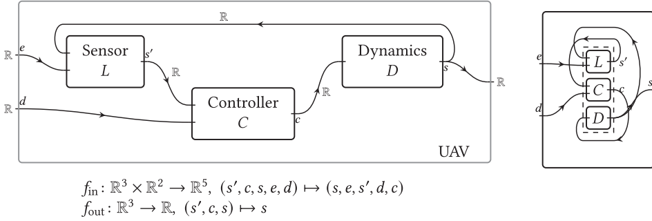
Fig. 3. The physical decomposition of the UAV, where d denotes the desired state, s' the predicted state, c the control action, s the current state, and e the environmental inputs.
